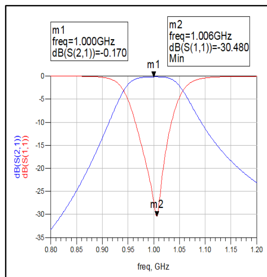
Fig.3: The ADS S-Parameters results of the Band pass filter value.
