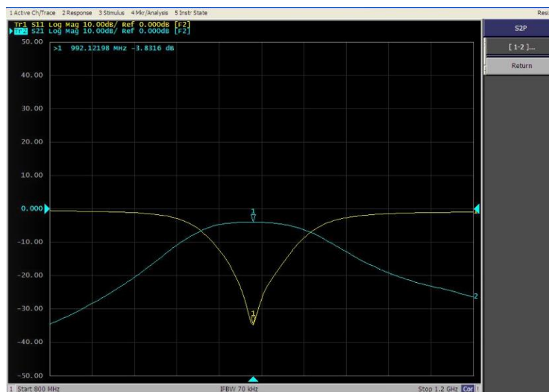
Fig.5: The fabrication experimental results for Band Pass Filter
