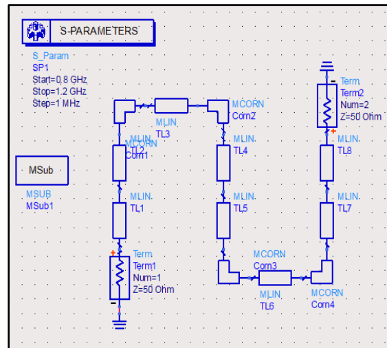
Fig.2: The schematic of lumped Band Pass Filter.
